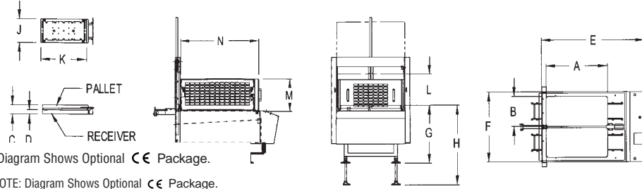
NOTE: Diagram Shows Optional CE Package.
